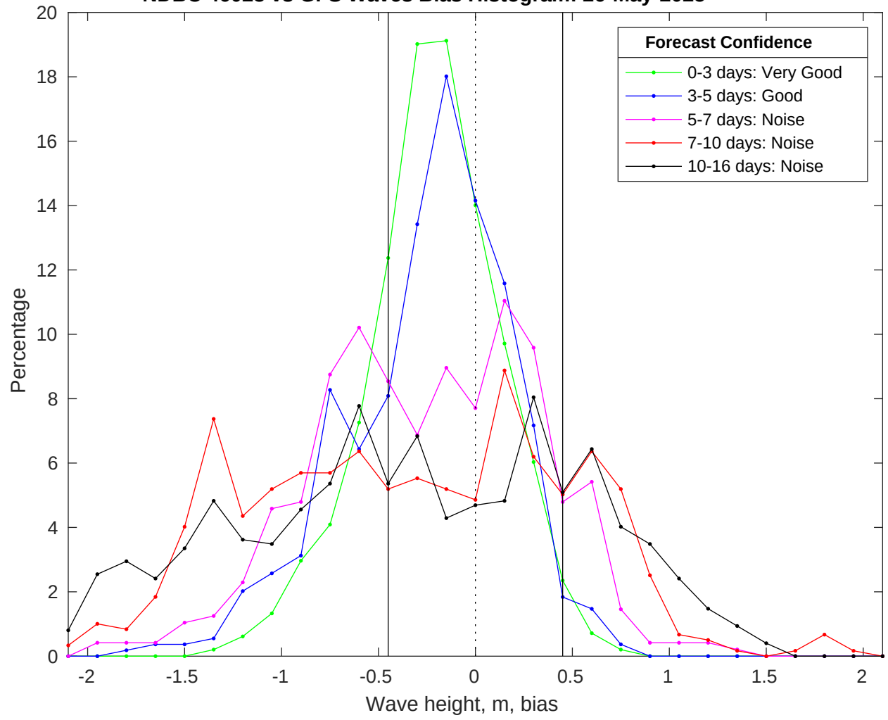
NDBC 46028 vs GFS Waves Bias Histogram: 26-May-2025
