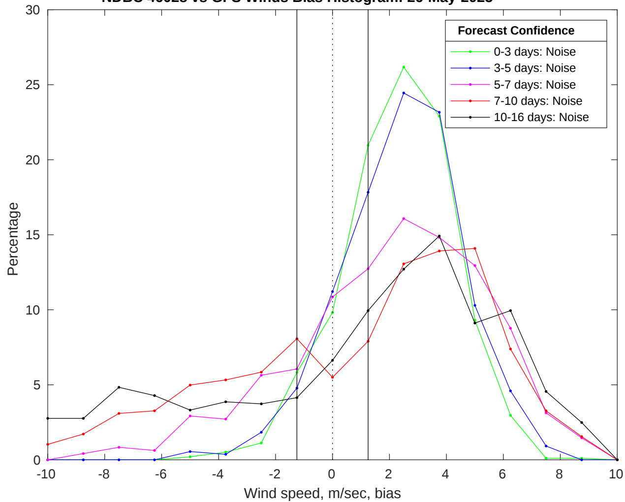
NDBC 46028 vs GFS Winds Bias Histogram: 26-May-2025
