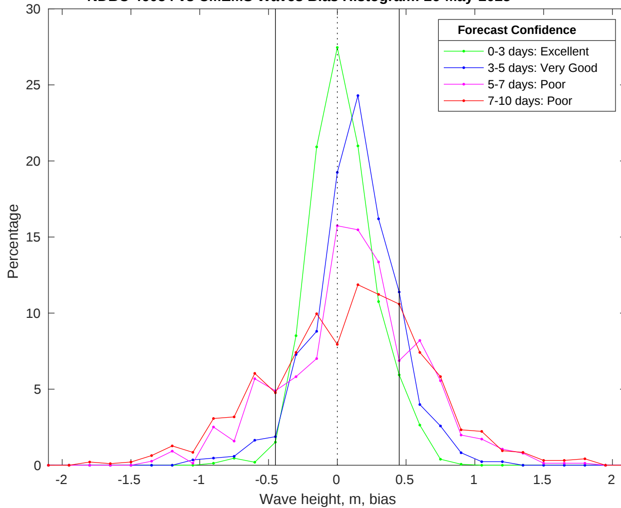
NDBC 46054 vs CMEMS Waves Bias Histogram: 26-May-2025
