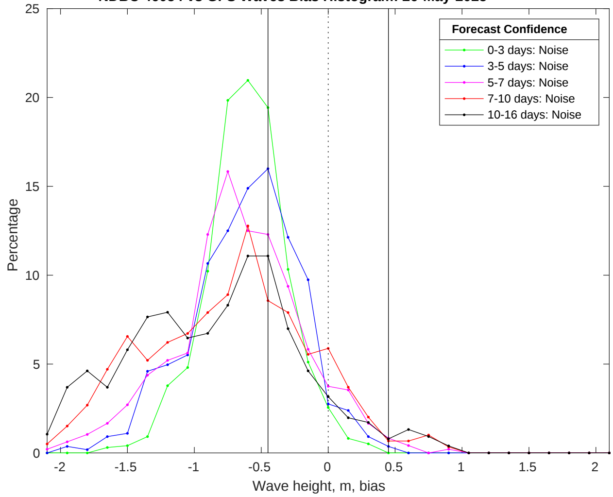
NDBC 46054 vs GFS Waves Bias Histogram: 26-May-2025
