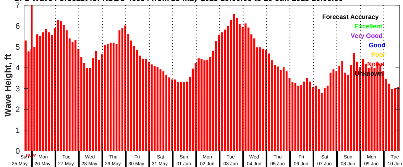
GFS Wave Forecast for NDBC 46054 from 25-May-2025 16:00:00 to 10-Jun-2025 16:00:00
