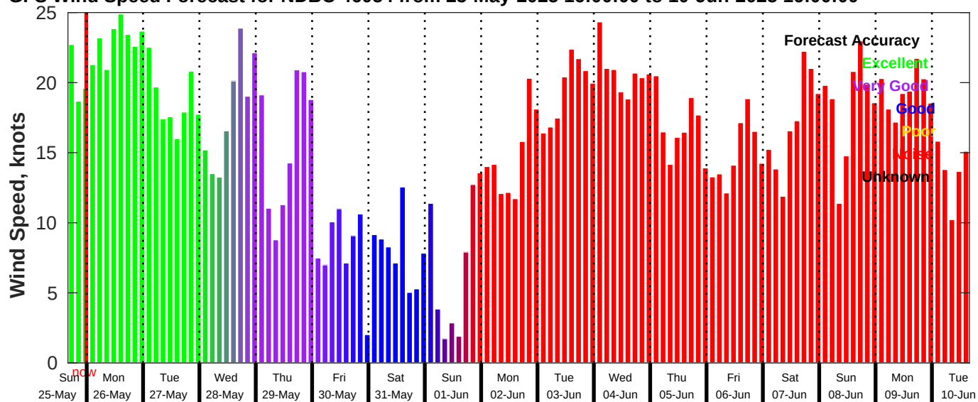
GFS Wind Speed Forecast for NDBC 46054 from 25-May-2025 16:00:00 to 10-Jun-2025 16:00:00
