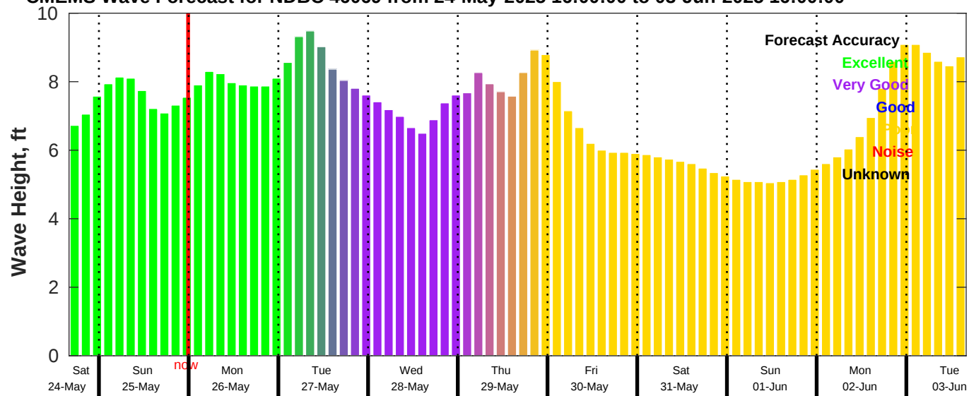
CMEMS Wave Forecast for NDBC 46069 from 24-May-2025 16:00:00 to 03-Jun-2025 16:00:00
