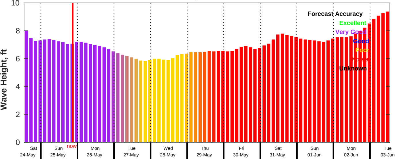
CMEMS Wave Forecast for NDBC 51209 from 24-May-2025 13:00:00 to 03-Jun-2025 13:00:00
