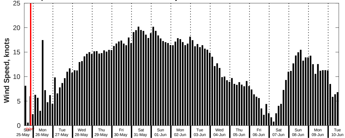
GFS Wind Speed Forecast for NDBC 51209 from 25-May-2025 13:00:00 to 10-Jun-2025 13:00:00
