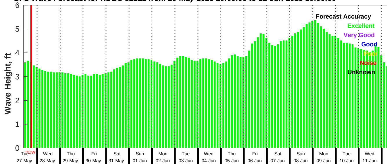
GFS Wave Forecast for NDBC 52211 from 26-May-2025 10:00:00 to 11-Jun-2025 10:00:00
