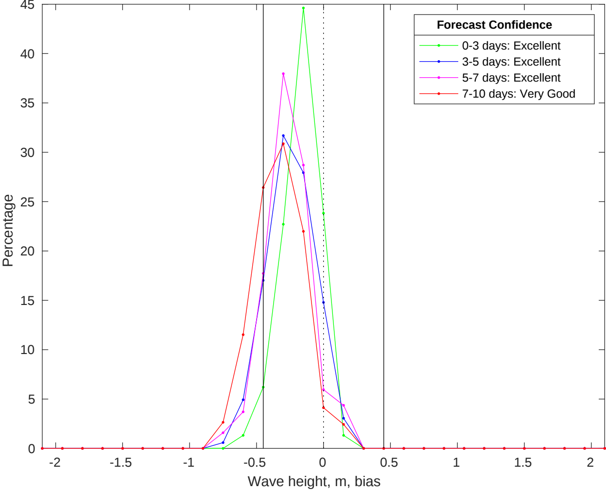
NDBC 52212 vs CMEMS Waves Bias Histogram: 26-May-2025
