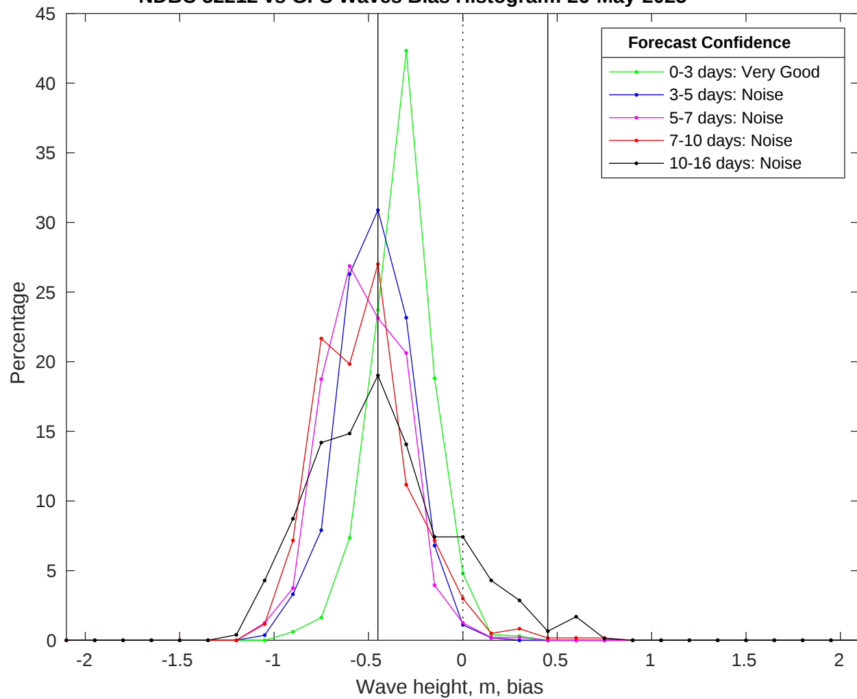
NDBC 52212 vs GFS Waves Bias Histogram: 26-May-2025
