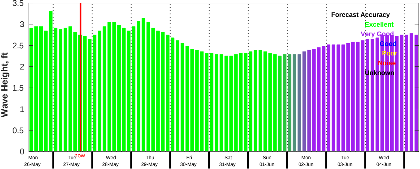
CMEMS Wave Forecast for NDBC 52212 from 25-May-2025 09:00:00 to 04-Jun-2025 09:00:00
