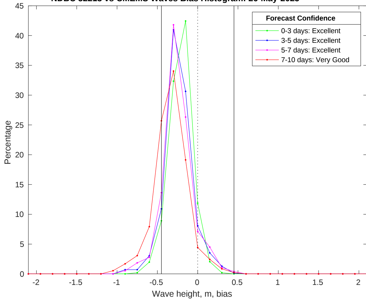
NDBC 52213 vs CMEMS Waves Bias Histogram: 26-May-2025
