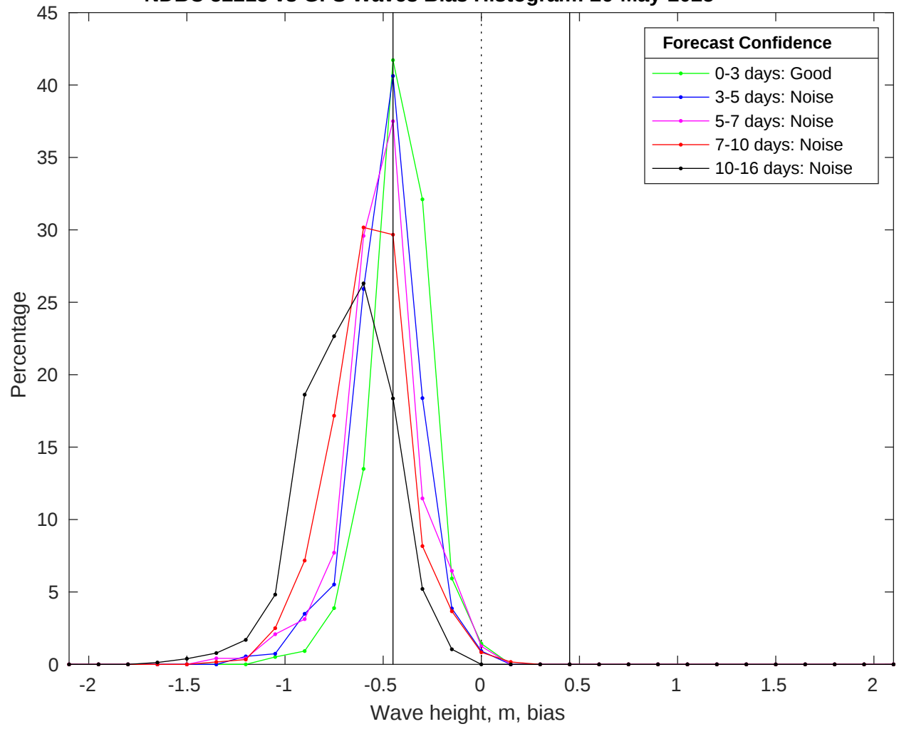
NDBC 52213 vs GFS Waves Bias Histogram: 26-May-2025
