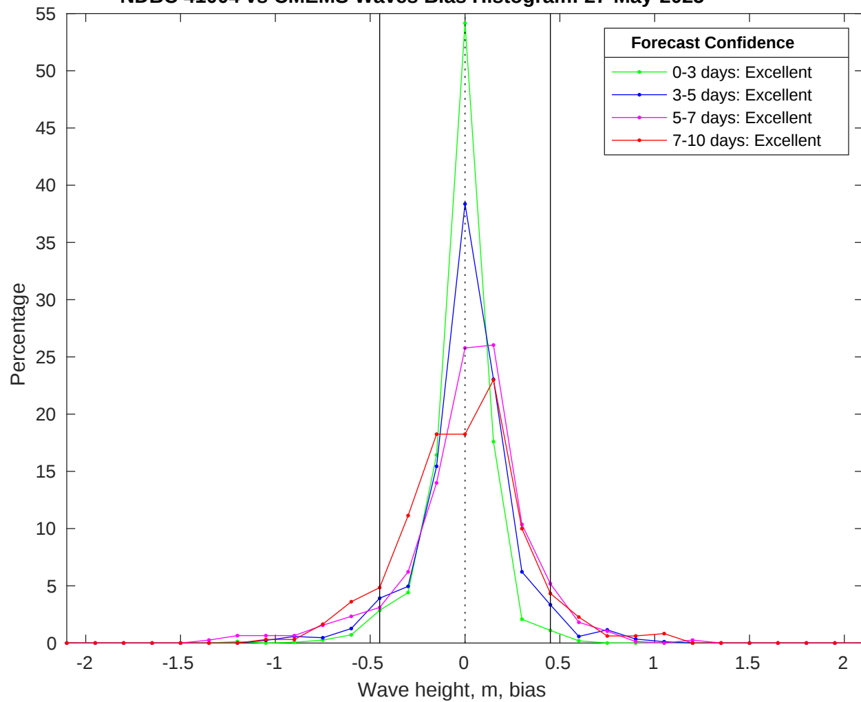
NDBC 41004 vs CMEMS Waves Bias Histogram: 27-May-2025
