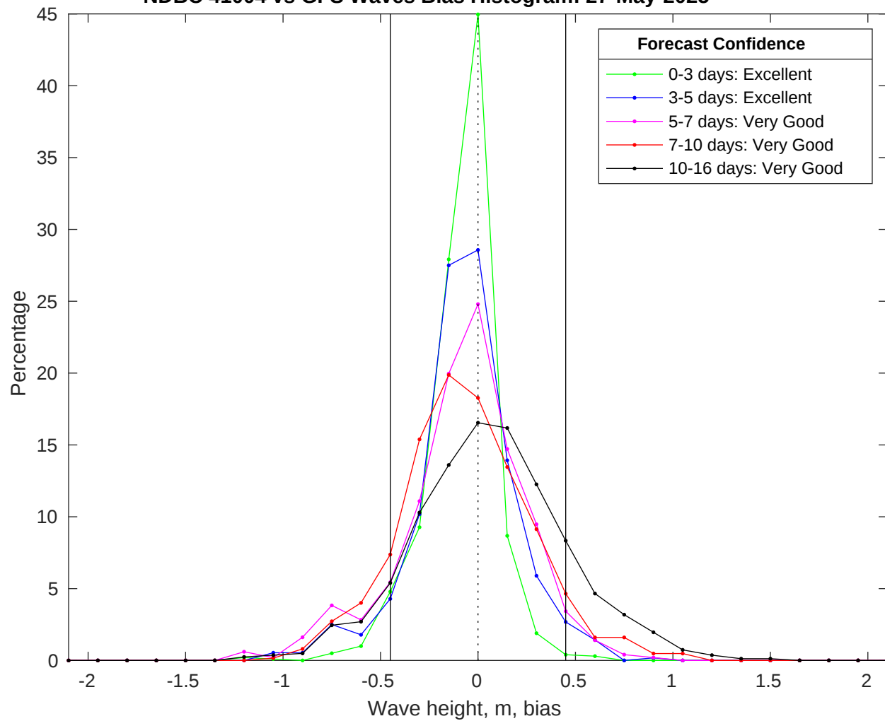
NDBC 41004 vs GFS Waves Bias Histogram: 27-May-2025
