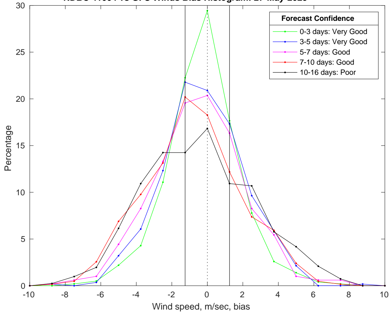
NDBC 41004 vs GFS Winds Bias Histogram: 27-May-2025
