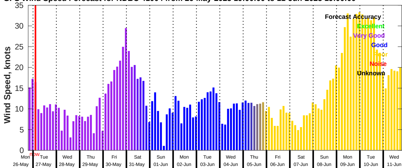
GFS Wind Speed Forecast for NDBC 41004 from 26-May-2025 19:00:00 to 11-Jun-2025 19:00:00
