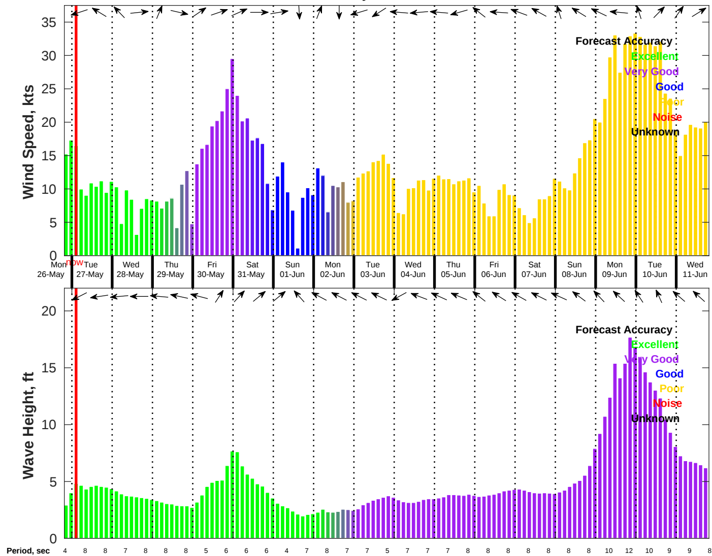
Wind & Wave Forecast for NDBC 41004 from 26-May-2025 19:00:00 to 11-Jun-2025 19:00:00
