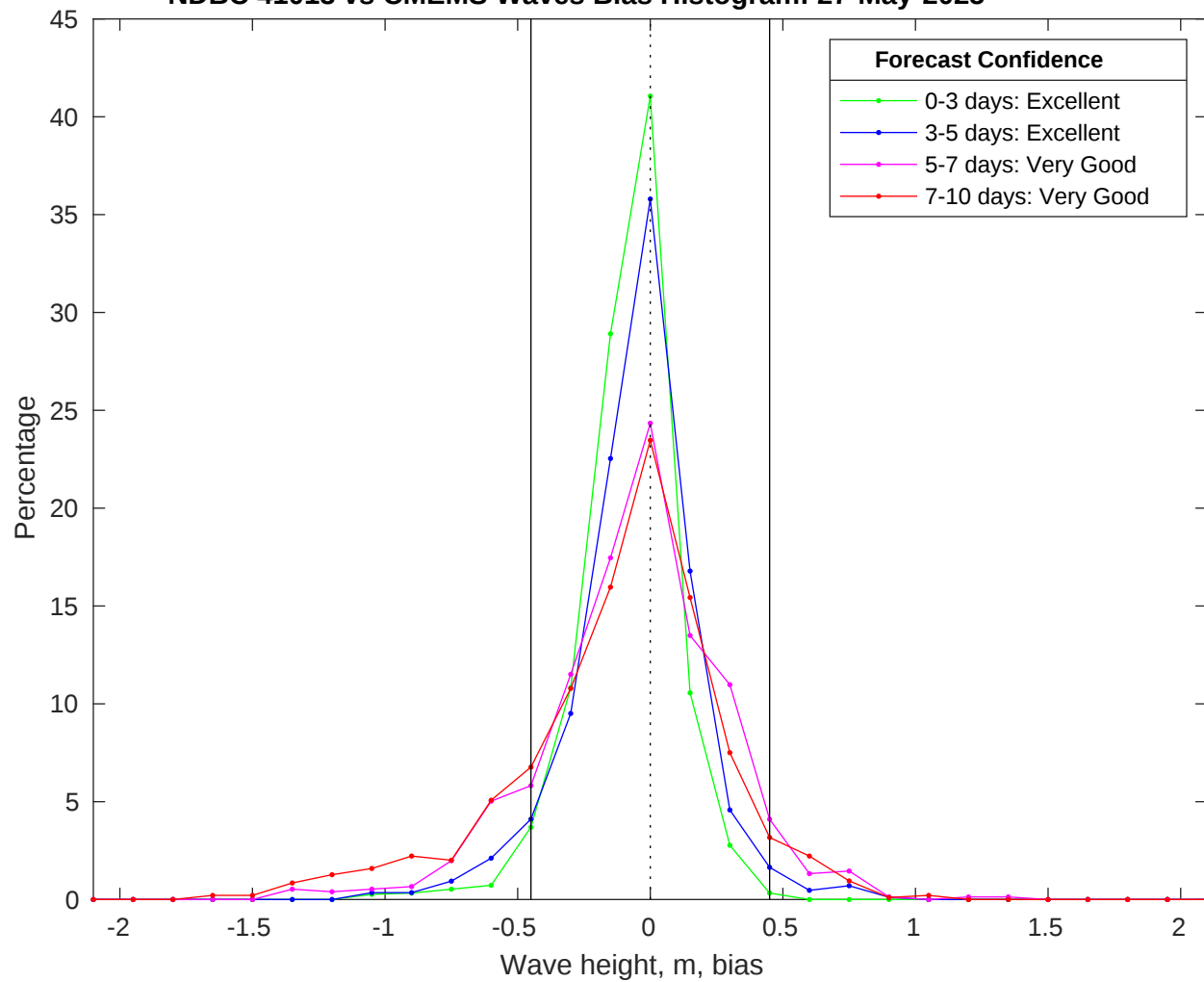
NDBC 41013 vs CMEMS Waves Bias Histogram: 27-May-2025
