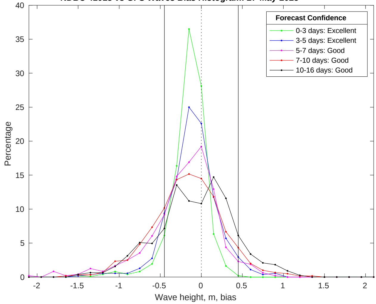
NDBC 41013 vs GFS Waves Bias Histogram: 27-May-2025
