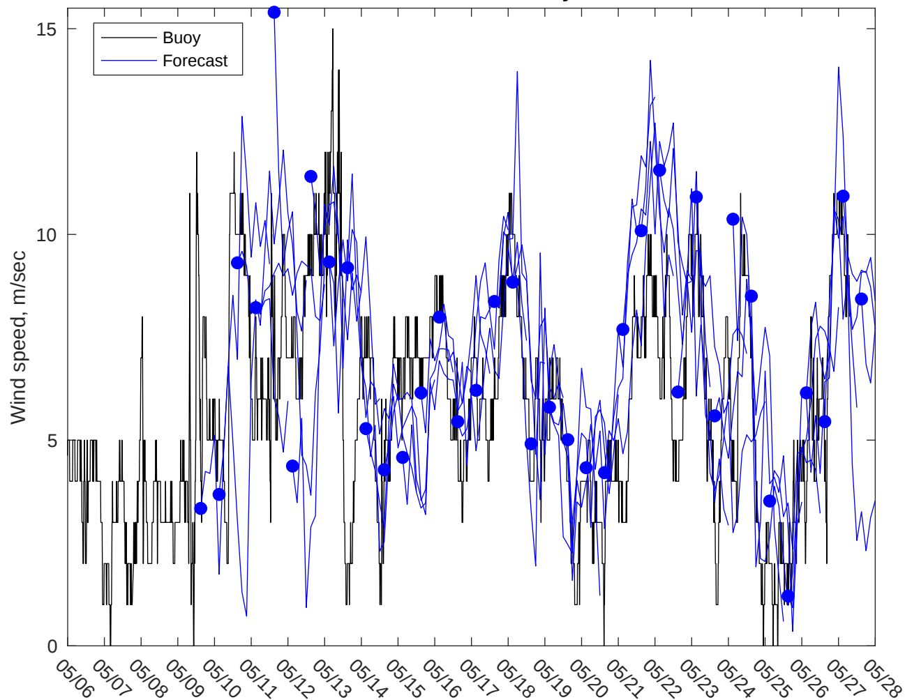
NDBC 41013 vs GFS Winds: 3 to 5 day forecast
