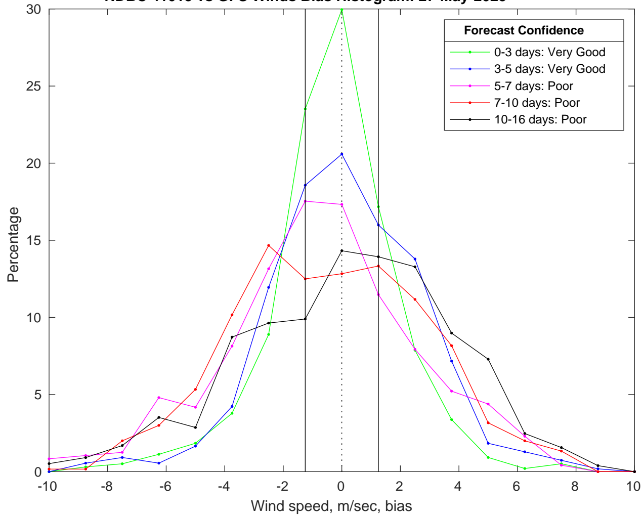
NDBC 41013 vs GFS Winds Bias Histogram: 27-May-2025
