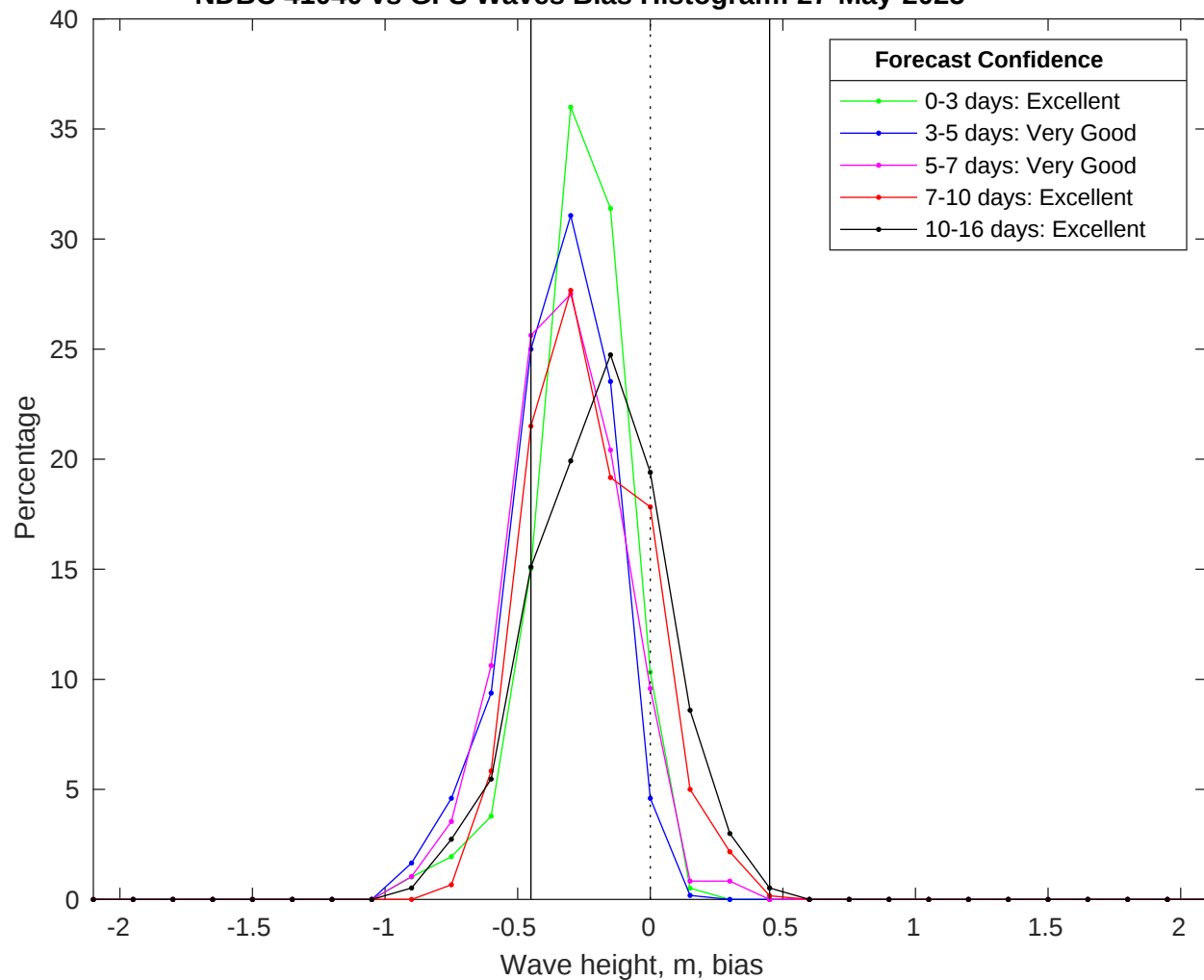
NDBC 41040 vs GFS Waves Bias Histogram: 27-May-2025
