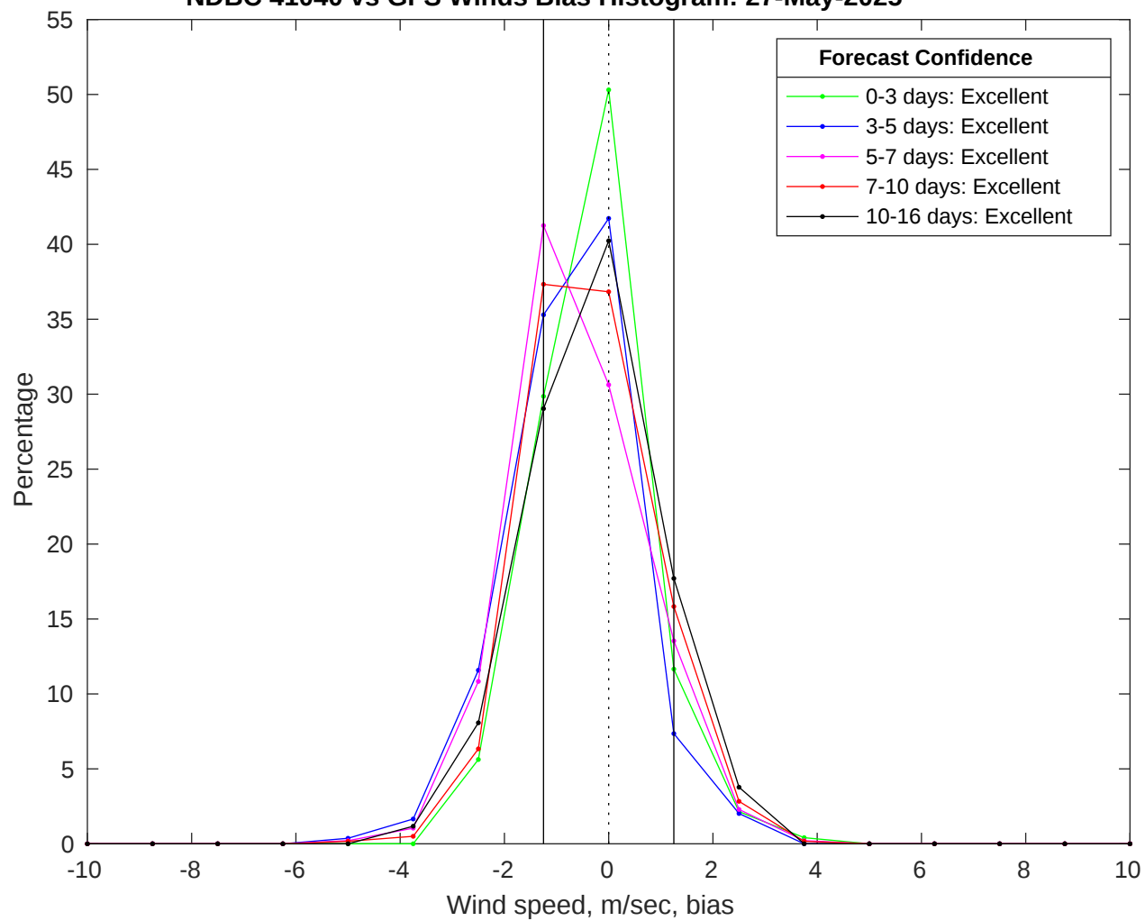
NDBC 41040 vs GFS Winds Bias Histogram: 27-May-2025
