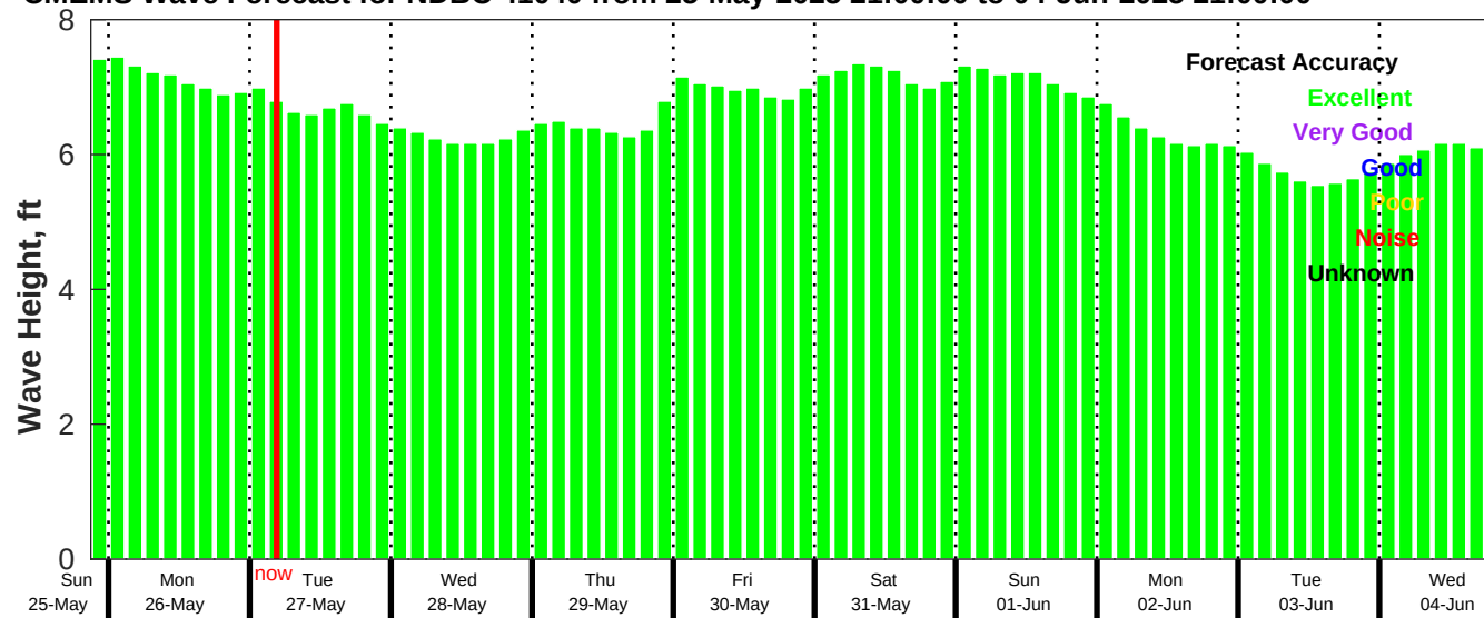
CMEMS Wave Forecast for NDBC 41040 from 25-May-2025 21:00:00 to 04-Jun-2025 21:00:00
