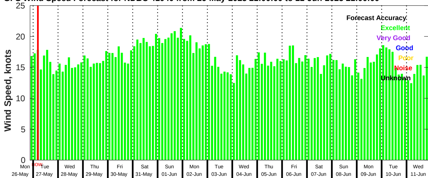
GFS Wind Speed Forecast for NDBC 41040 from 26-May-2025 21:00:00 to 11-Jun-2025 21:00:00
