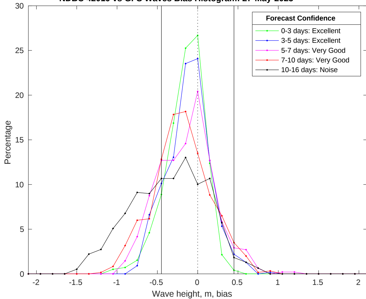
NDBC 42019 vs GFS Waves Bias Histogram: 27-May-2025
