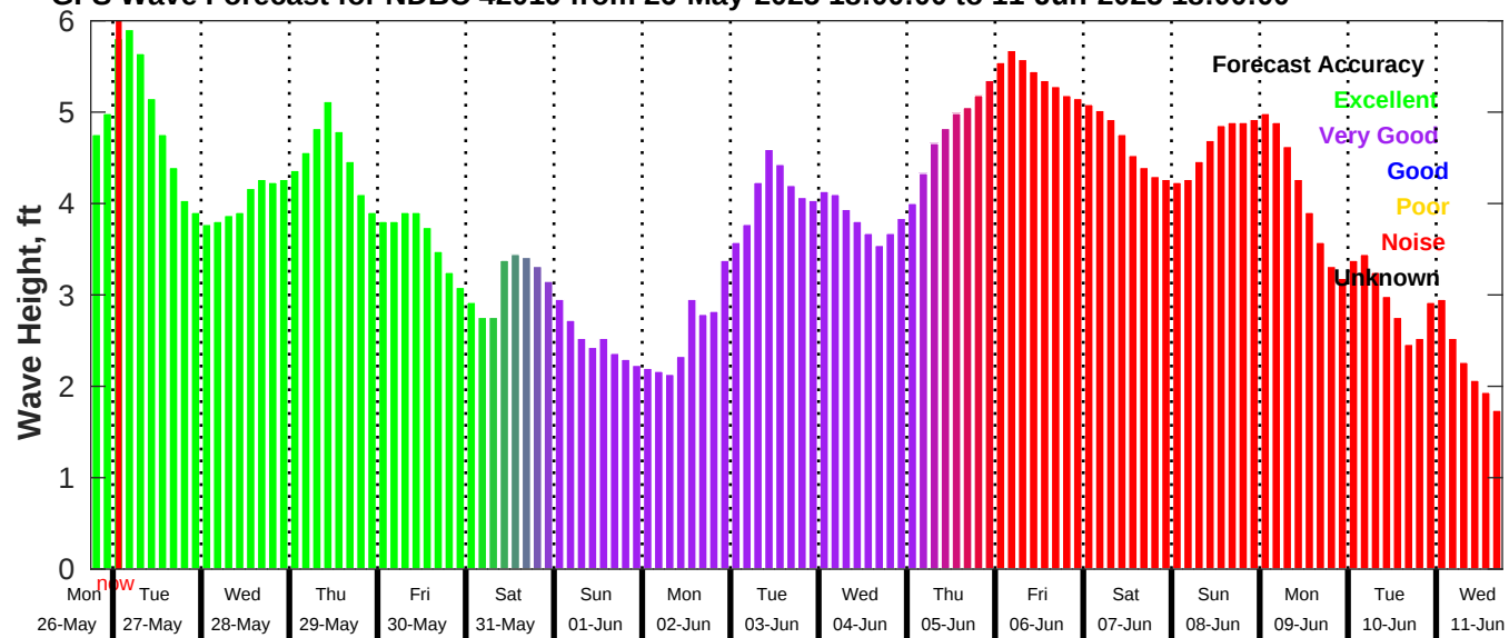
GFS Wave Forecast for NDBC 42019 from 26-May-2025 18:00:00 to 11-Jun-2025 18:00:00
