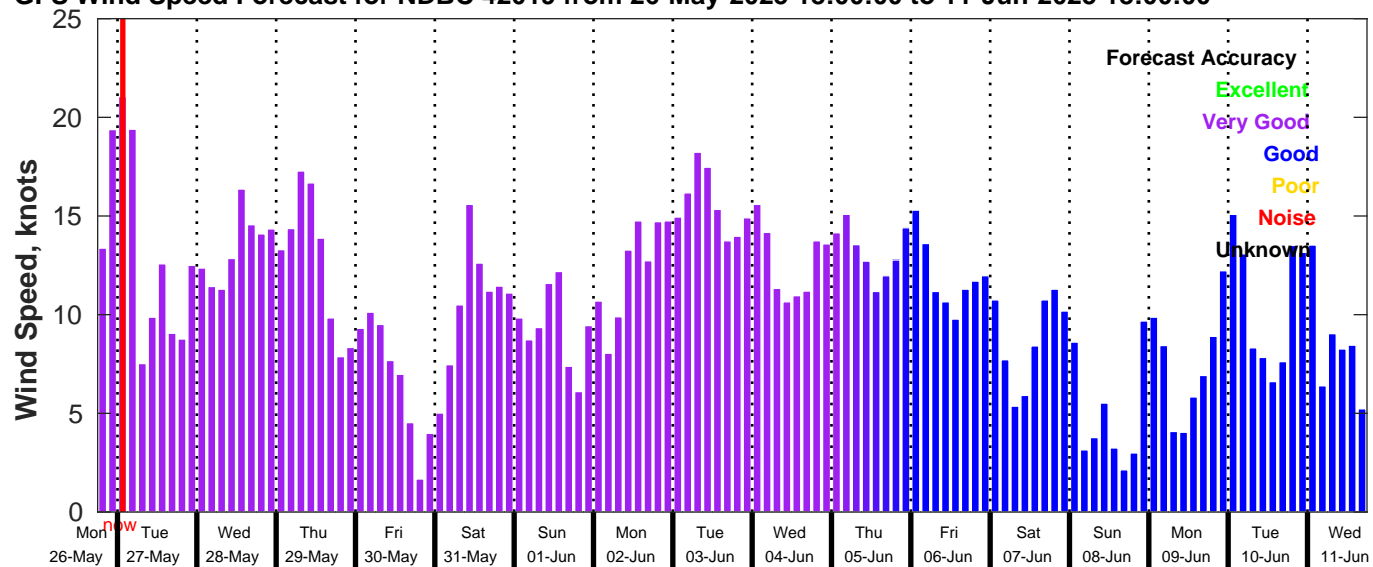
GFS Wind Speed Forecast for NDBC 42019 from 26-May-2025 18:00:00 to 11-Jun-2025 18:00:00
