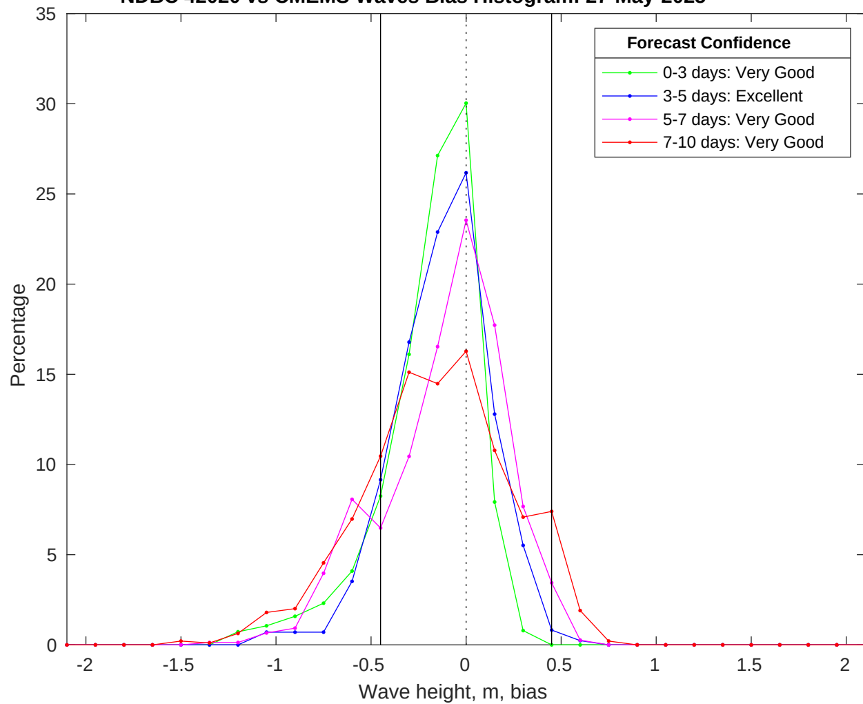
NDBC 42020 vs CMEMS Waves Bias Histogram: 27-May-2025
