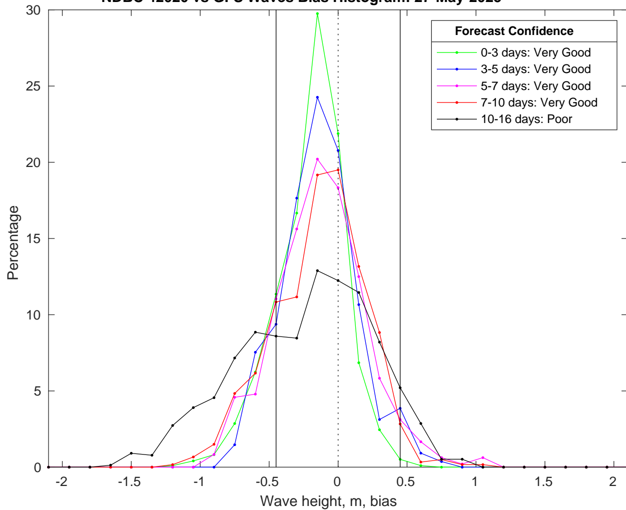
NDBC 42020 vs GFS Waves Bias Histogram: 27-May-2025
