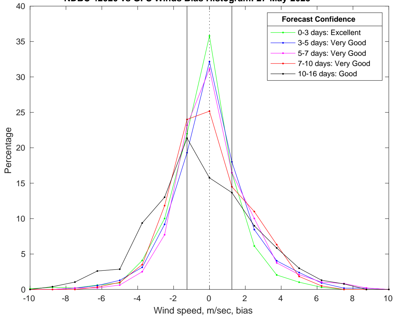
NDBC 42020 vs GFS Winds Bias Histogram: 27-May-2025
