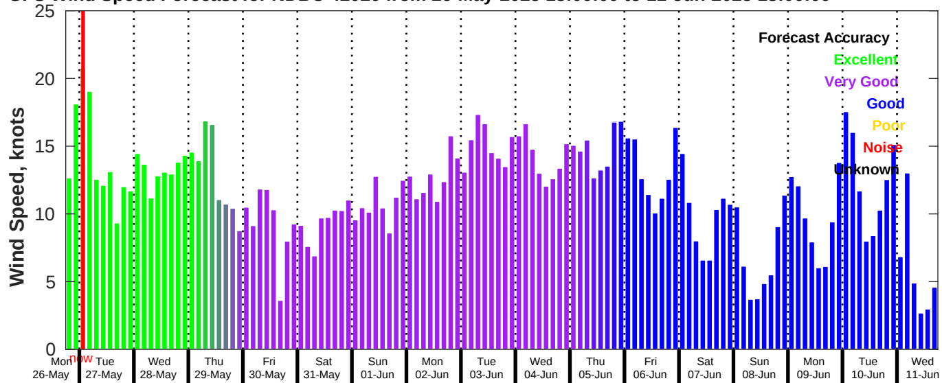
GFS Wind Speed Forecast for NDBC 42020 from 26-May-2025 18:00:00 to 11-Jun-2025 18:00:00
