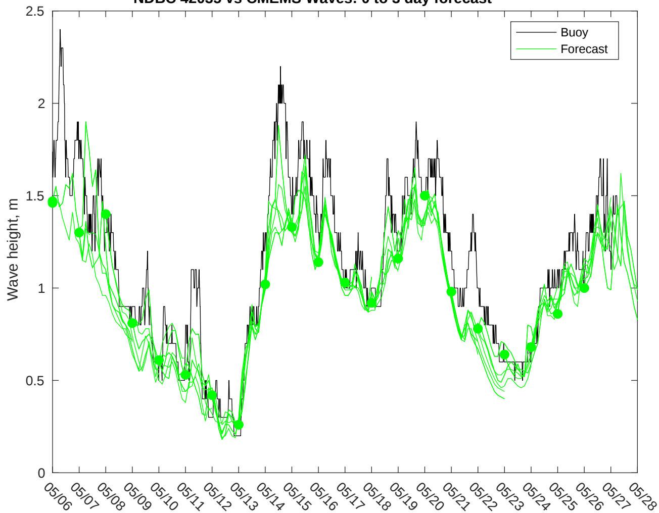
NDBC 42035 vs CMEMS Waves: 0 to 3 day forecast
