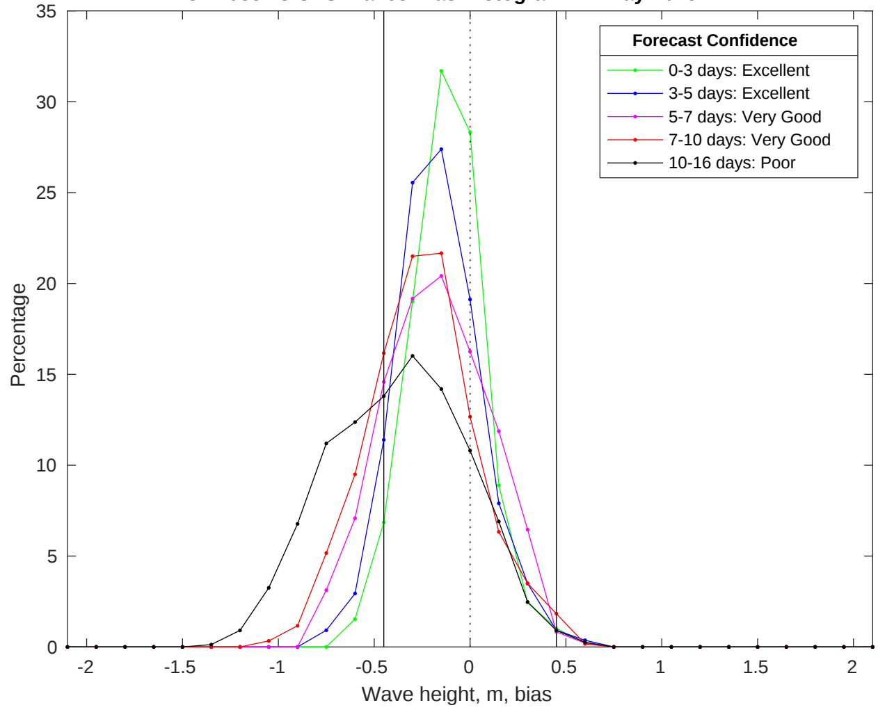
NDBC 42035 vs GFS Waves Bias Histogram: 27-May-2025
