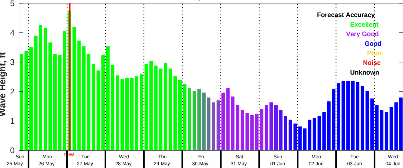
CMEMS Wave Forecast for NDBC 42035 from 25-May-2025 18:00:00 to 04-Jun-2025 18:00:00
