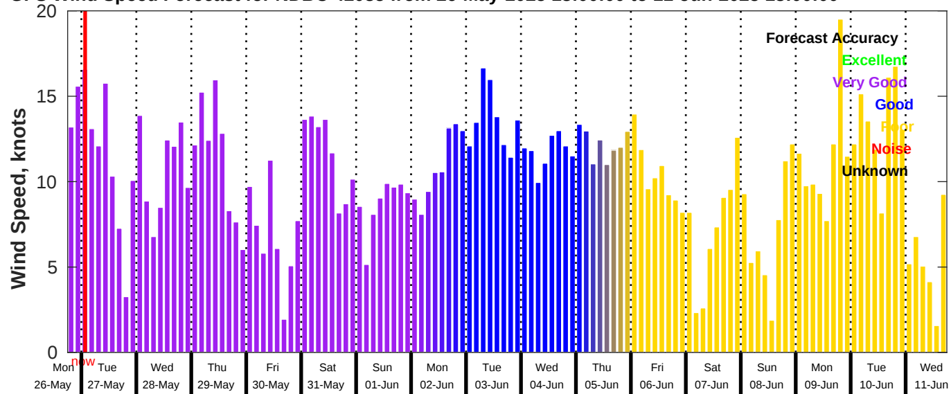
GFS Wind Speed Forecast for NDBC 42035 from 26-May-2025 18:00:00 to 11-Jun-2025 18:00:00
