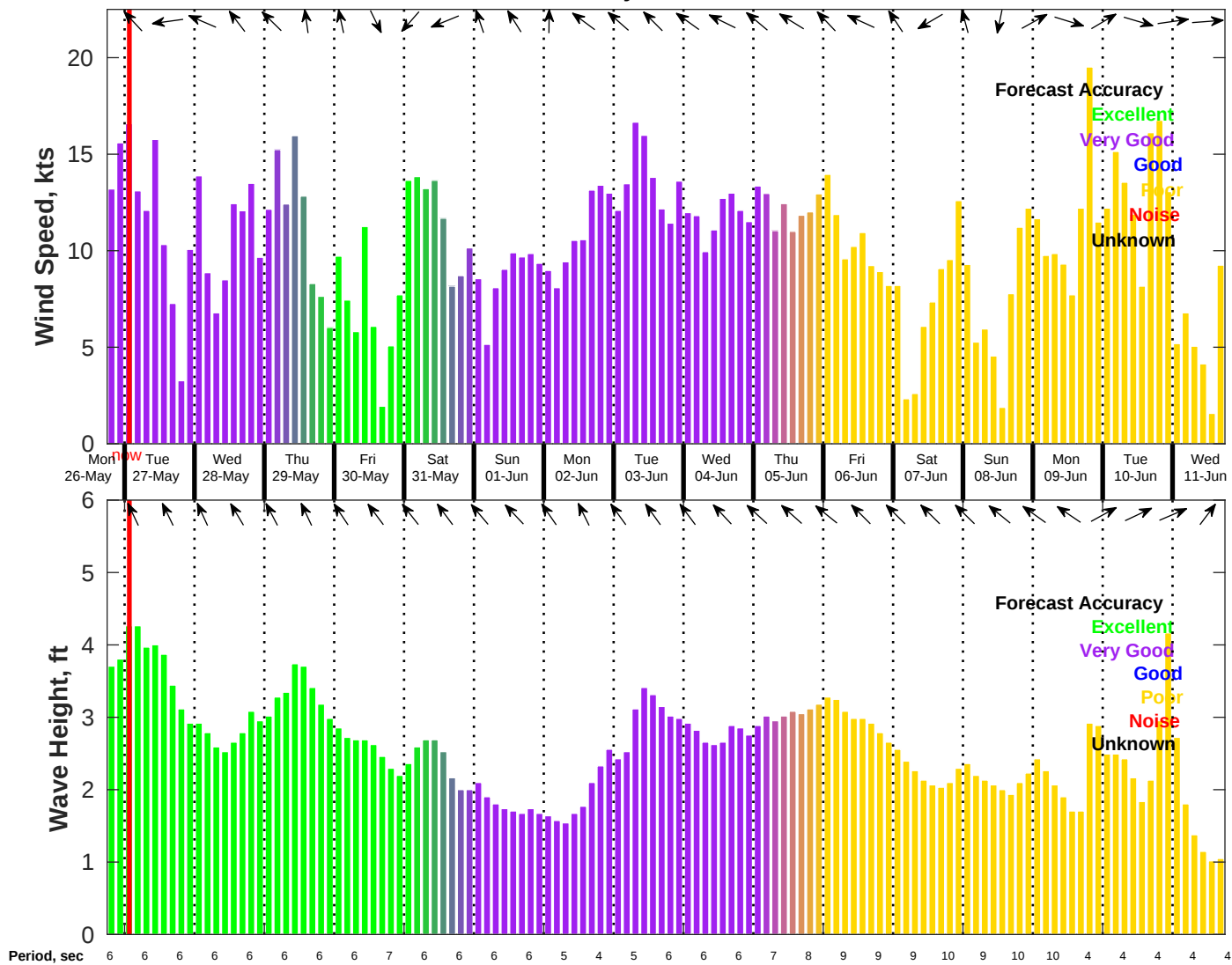
Wind & Wave Forecast for NDBC 42035 from 26-May-2025 18:00:00 to 11-Jun-2025 18:00:00
