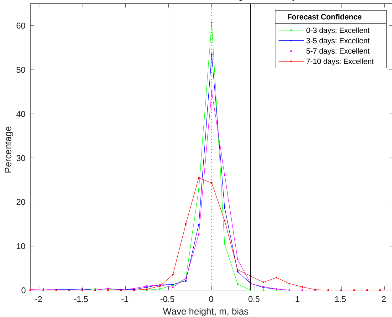
NDBC 42036 vs CMEMS Waves Bias Histogram: 27-May-2025
