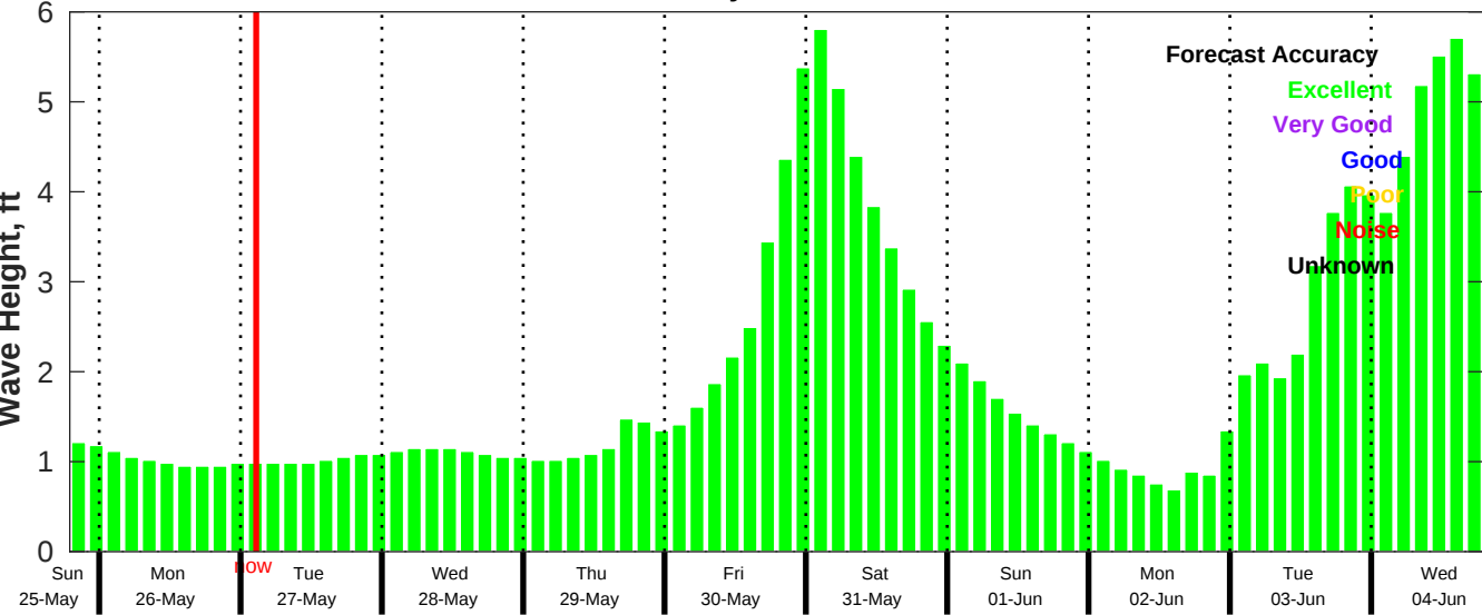
CMEMS Wave Forecast for NDBC 42036 from 25-May-2025 19:00:00 to 04-Jun-2025 19:00:00
