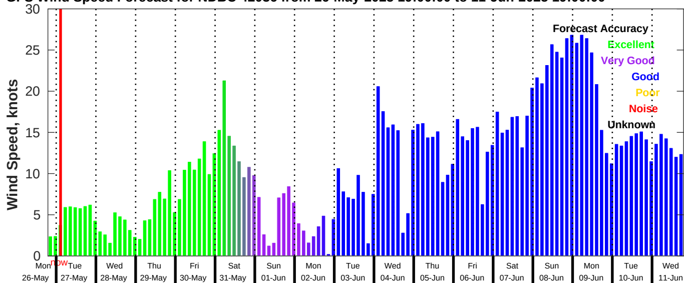
GFS Wind Speed Forecast for NDBC 42036 from 26-May-2025 19:00:00 to 11-Jun-2025 19:00:00
