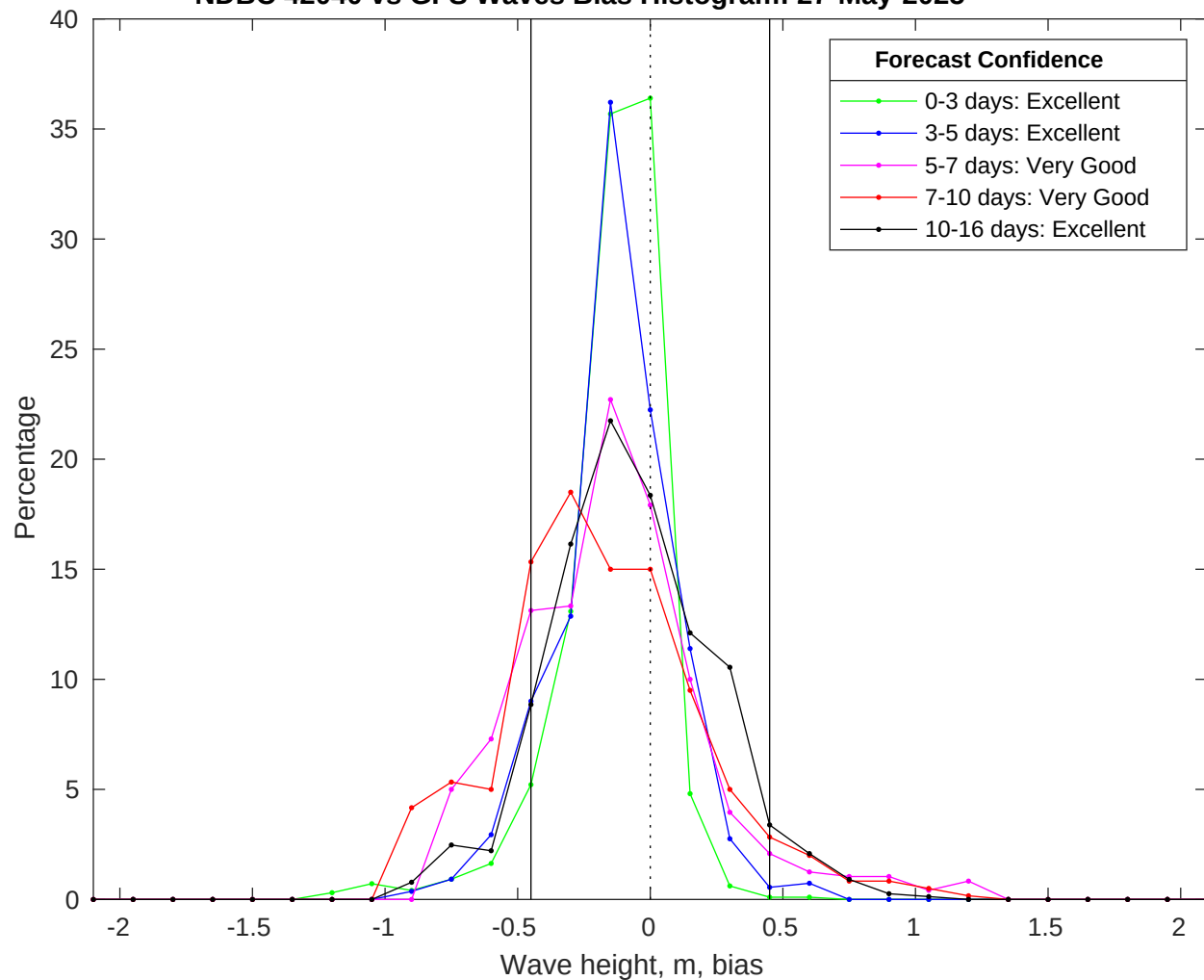
NDBC 42040 vs GFS Waves Bias Histogram: 27-May-2025
