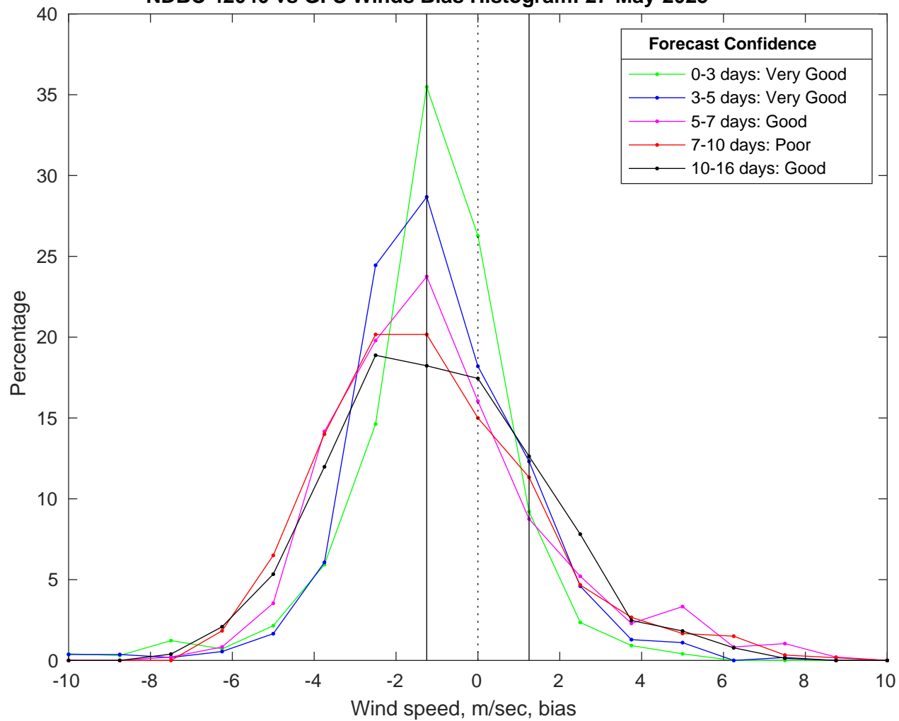
NDBC 42040 vs GFS Winds Bias Histogram: 27-May-2025
