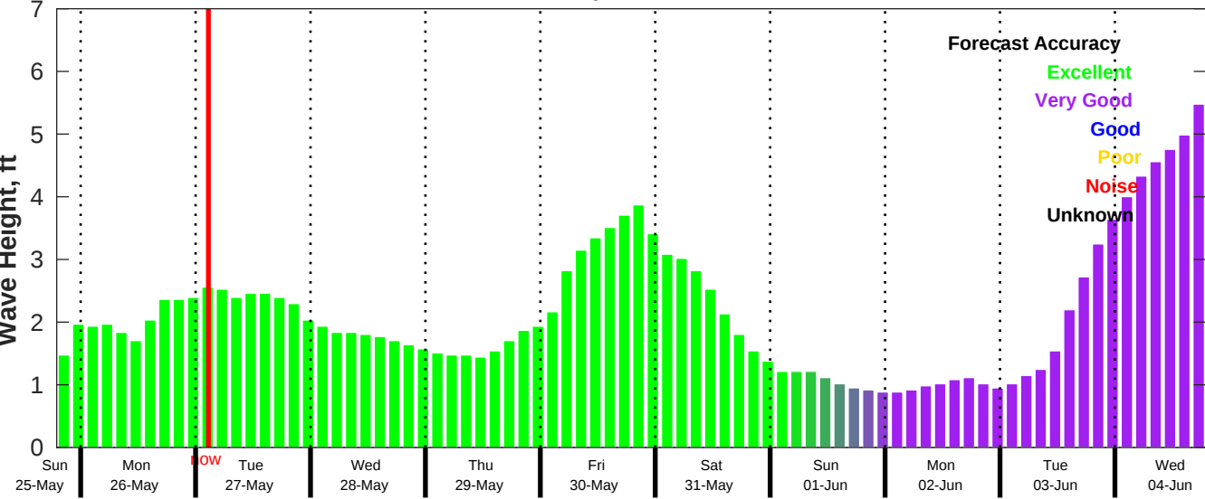
CMEMS Wave Forecast for NDBC 42040 from 25-May-2025 19:00:00 to 04-Jun-2025 19:00:00
