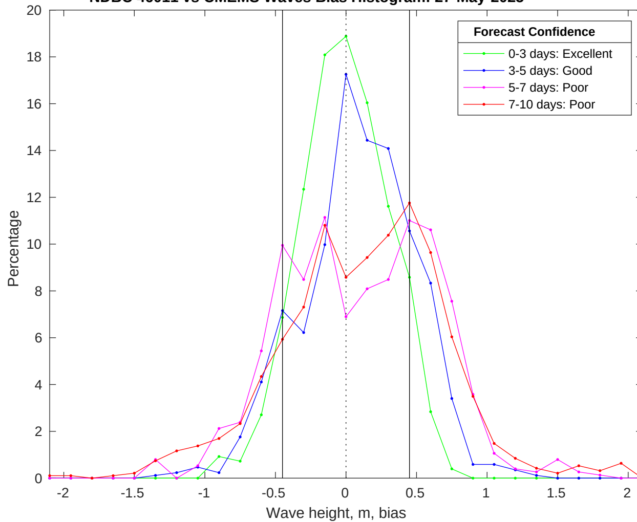
NDBC 46011 vs CMEMS Waves Bias Histogram: 27-May-2025
