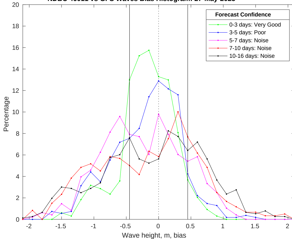
NDBC 46011 vs GFS Waves Bias Histogram: 27-May-2025
