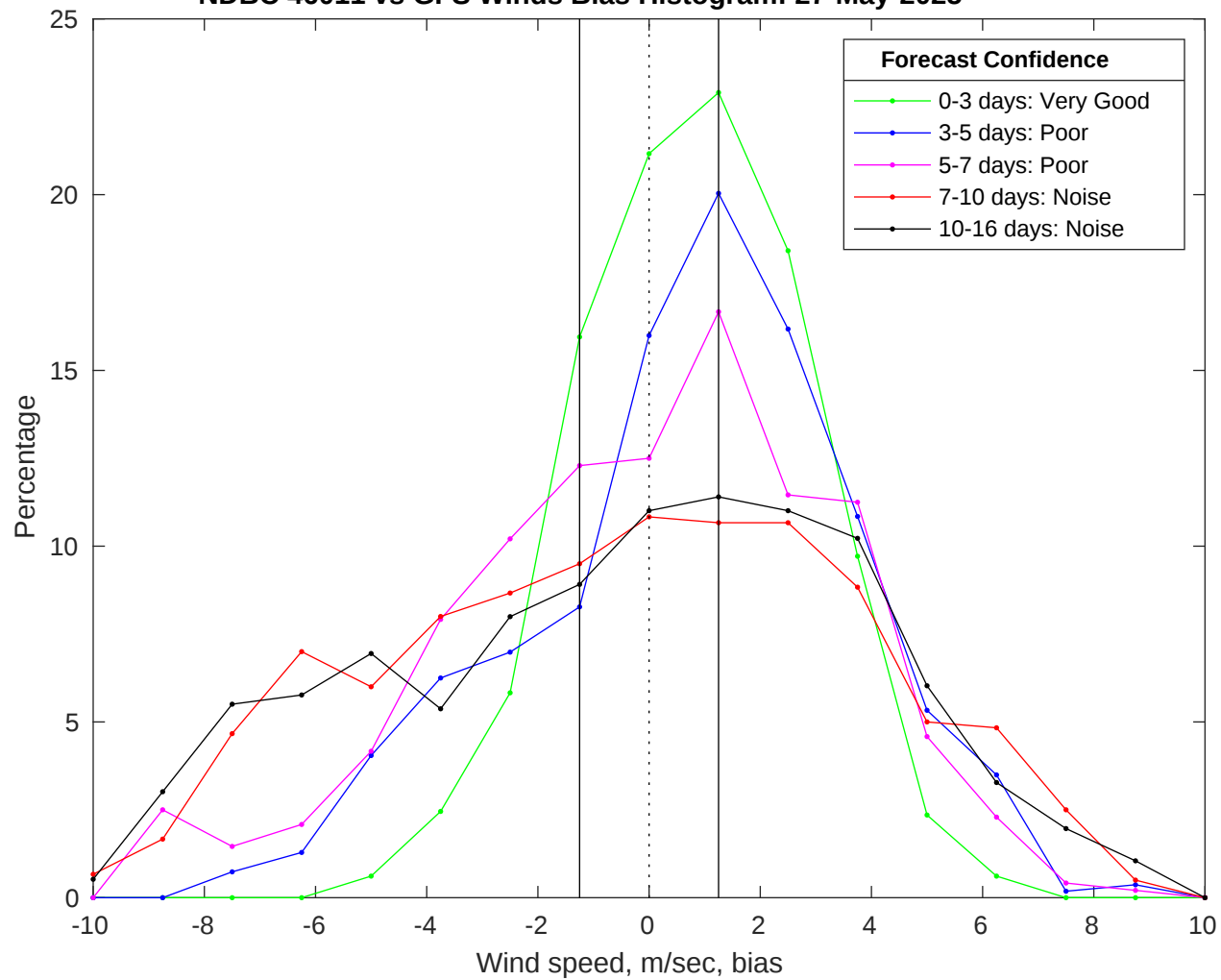
NDBC 46011 vs GFS Winds Bias Histogram: 27-May-2025
