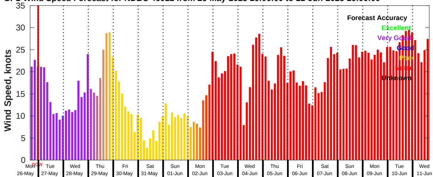
GFS Wind Speed Forecast for NDBC 46011 from 26-May-2025 16:00:00 to 11-Jun-2025 16:00:00
